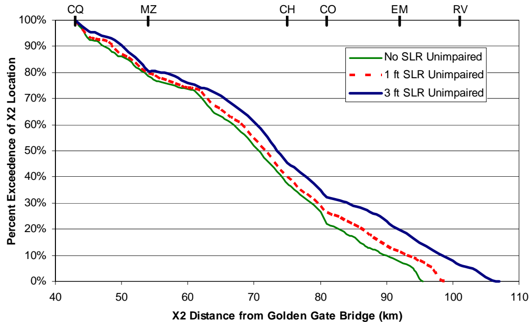
Figure 3 Effects of sea level rise on salinity intrusion for unimpaired flows. CQ – Carquinez Strait, MZ – Martinez Bridge, CH – Chipps Island, CO – Collinsville, EM – Emmaton, RV – Rio Vista
